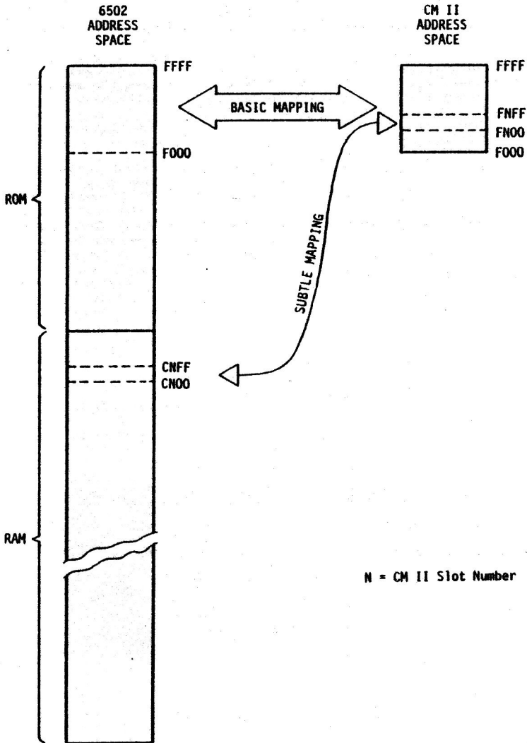
Figure 1: Diagram of Memory Mappings
